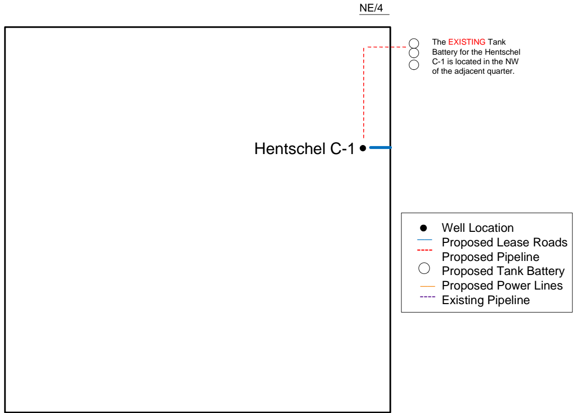
Proposed Details of NE/4 Sec 8 -T33S -R42W
