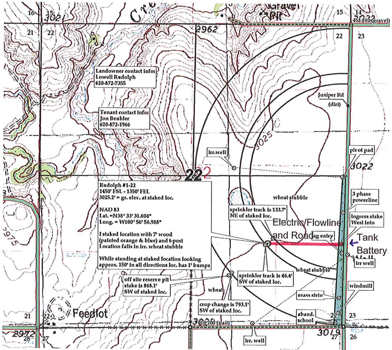
Preliminary non-bind estimate of tanks, flowlines and roads.
