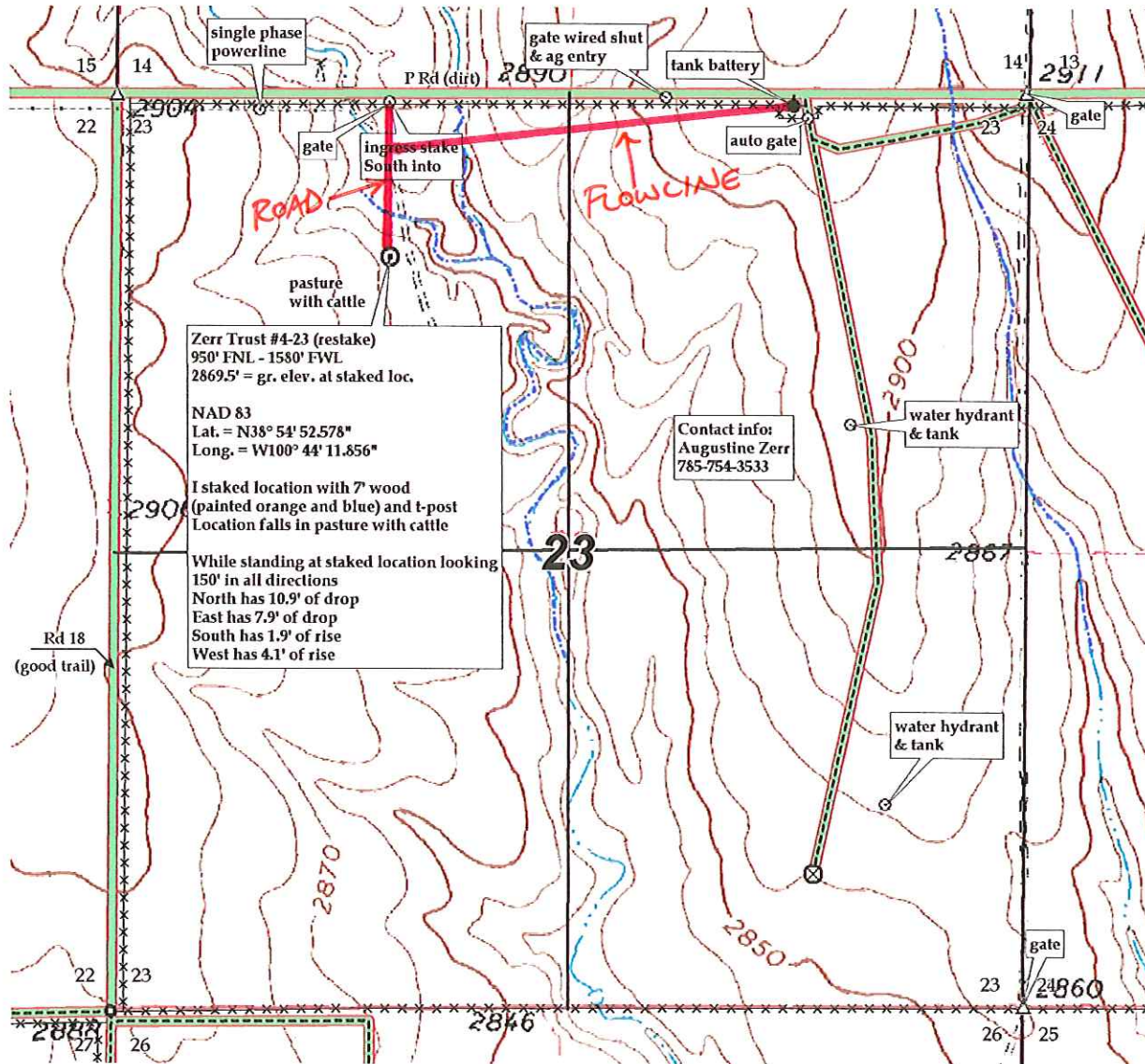
Preliminary non-binding estimate of flowlines, tanks and roads.
