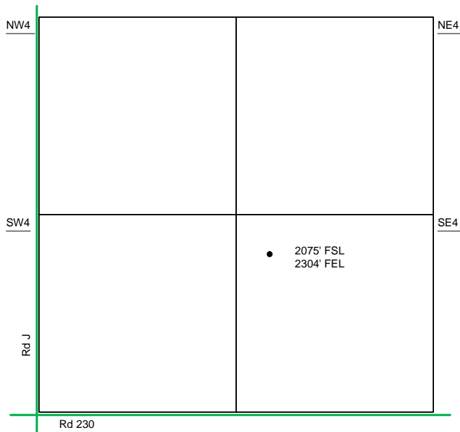
Sec 28 - T23S - R37W
