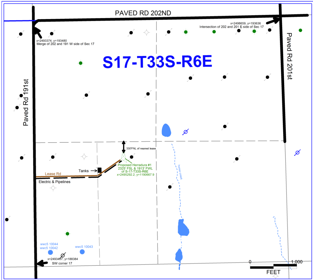
Tank and Road Locations for the Proposed Herradura #1 Sec 17- Twn 33S – Rng 6E
