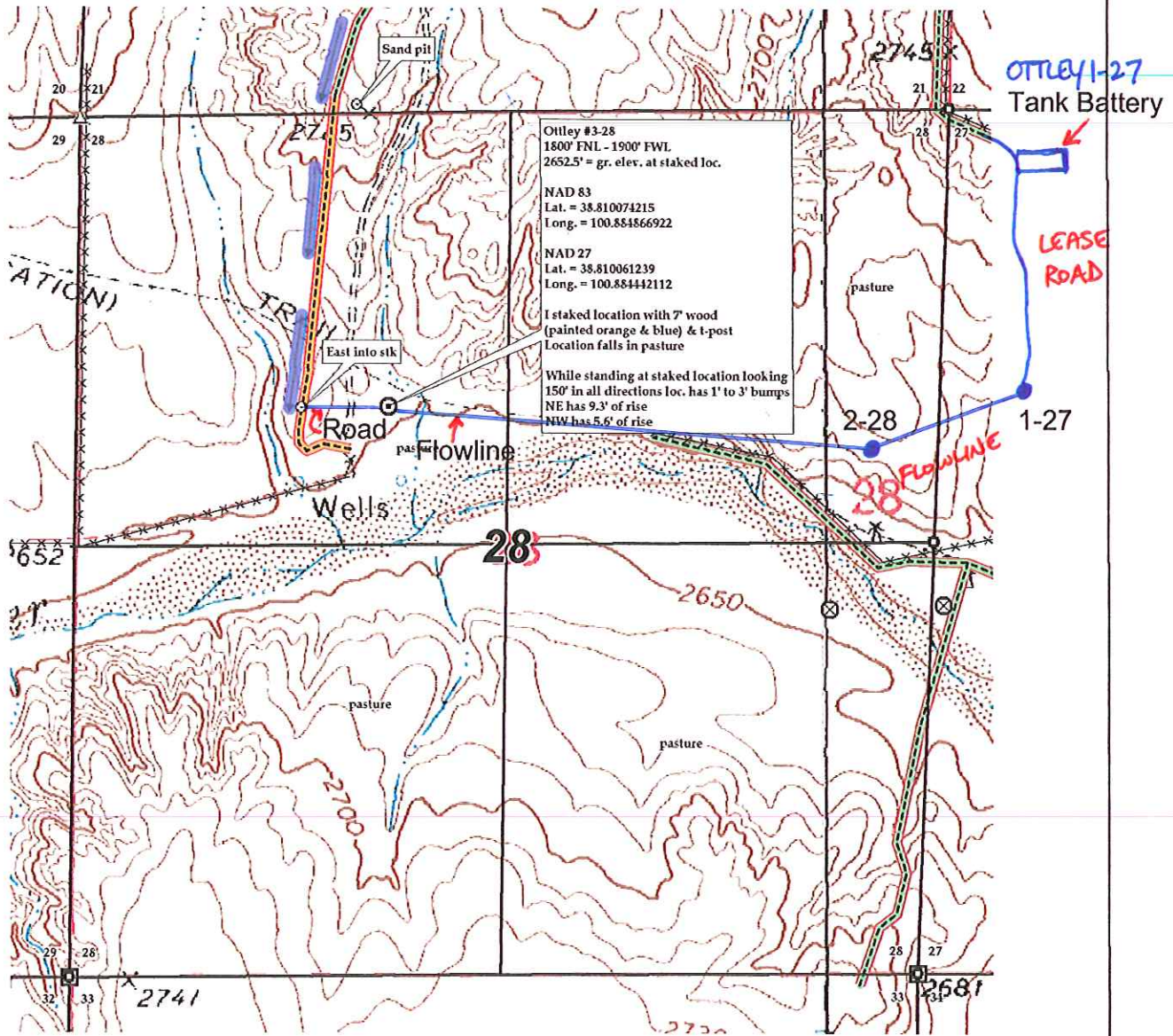
Preliminary non-binding estimate of flowlines, roads & tanks
