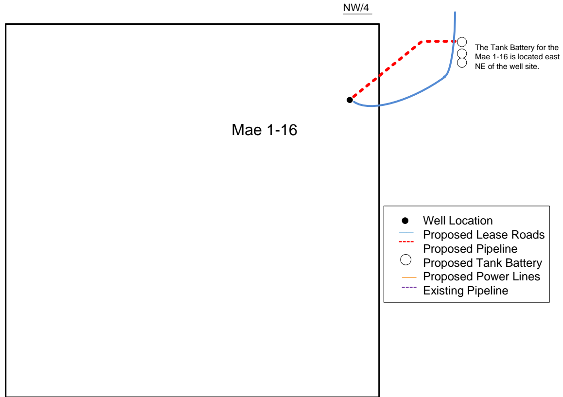
Proposed Details of NW/4 Sec 16 -T24S -R33W
