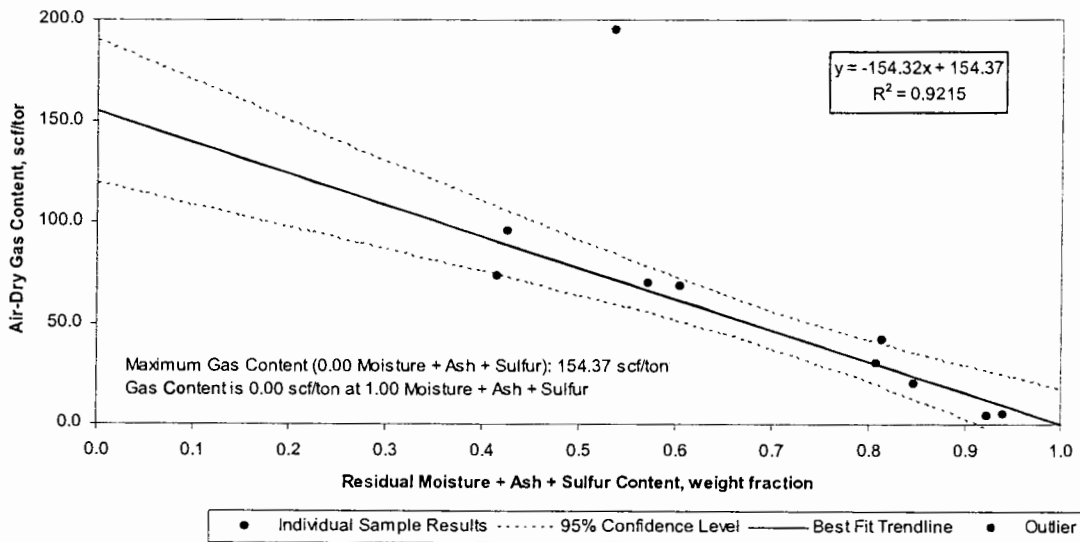
Figure 4-1 Sorbed Gas Content (Air-dry basis) versus Residual Moisture, Ash, and Total Sulfur for the Fuqua and Burch wells
