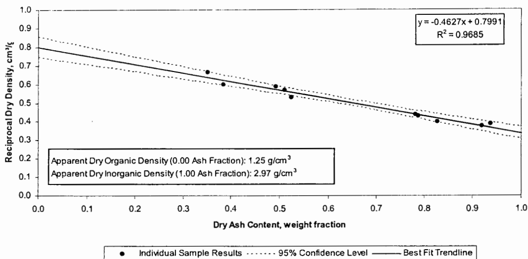
Figure 4-5 Variation of Reciprocal Helium Density versus Ash Content (Dry Basis) for the Fuqua and Burch wells
