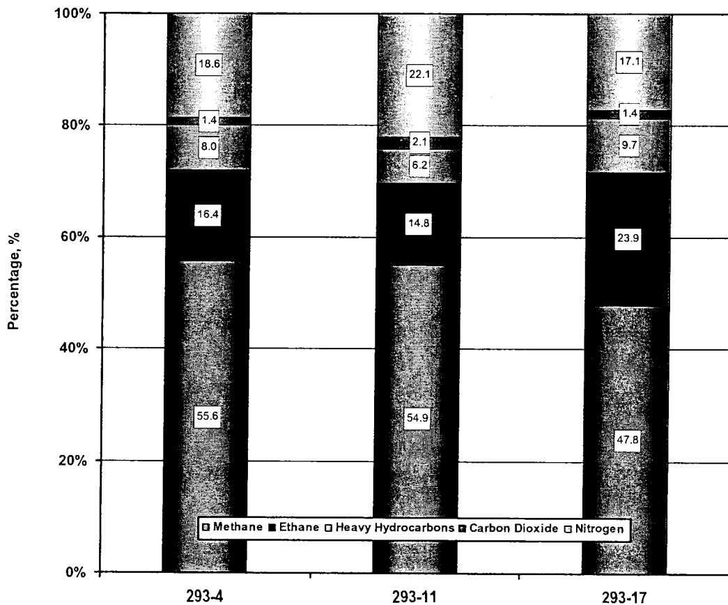
Figure 4-3 Apparent Sorbed Gas Composition
