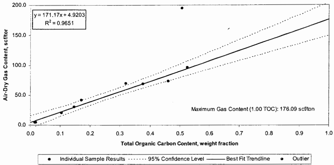
Figure 4-2 Sorbed Gas Content (Air-dry basis) versus Total Organic Carbon for the Fuqua and Burch wells
