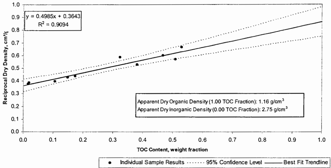
Figure 4-6 Variation of Reciprocal Helium Density versus Total Organic Carbon Content (Dry Basis) for the Fuqua and Burch wells
