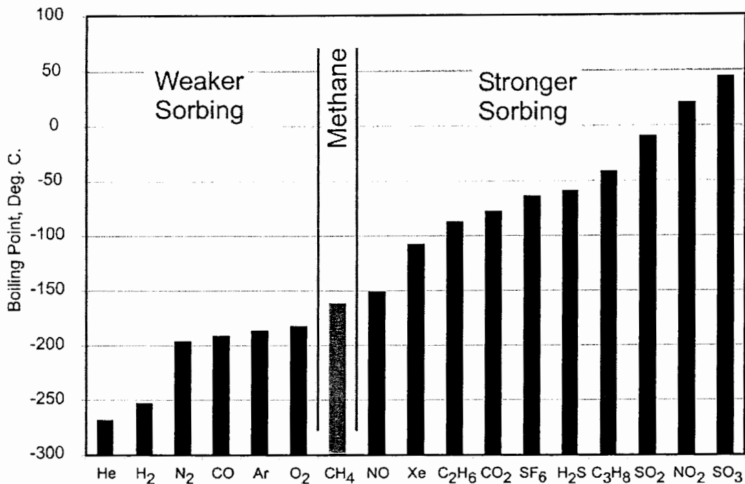
Figure 4-4 Relative Sorption Affinity of Gases Based on Boiling Point
