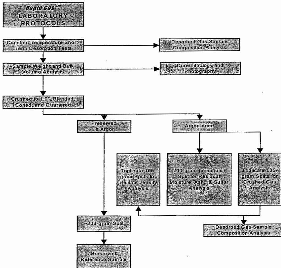
Figure 3-1 Flowchart of Sample Processing and Analysis
