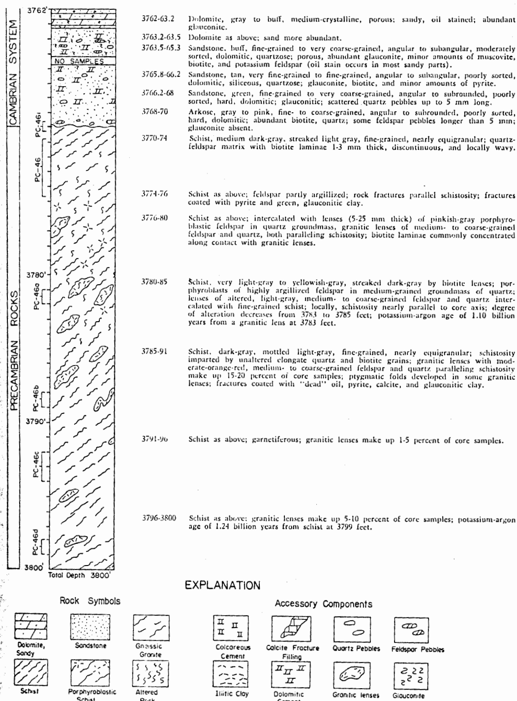
FIGURE 4.—Basal Arbuckle Group (3762-3763 feet), basal Paleozoic sandstone (3763-3770 feet), and Precambrian schist (3770-3800 feet) from Derby No. 4 Schoen well, C-SE sec. 35, T 3 S, R 24 W, Norton County, Kansas. (Thin section numbers are indicated along left margin of lithologic column.)
